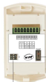
DIP SWITCH
